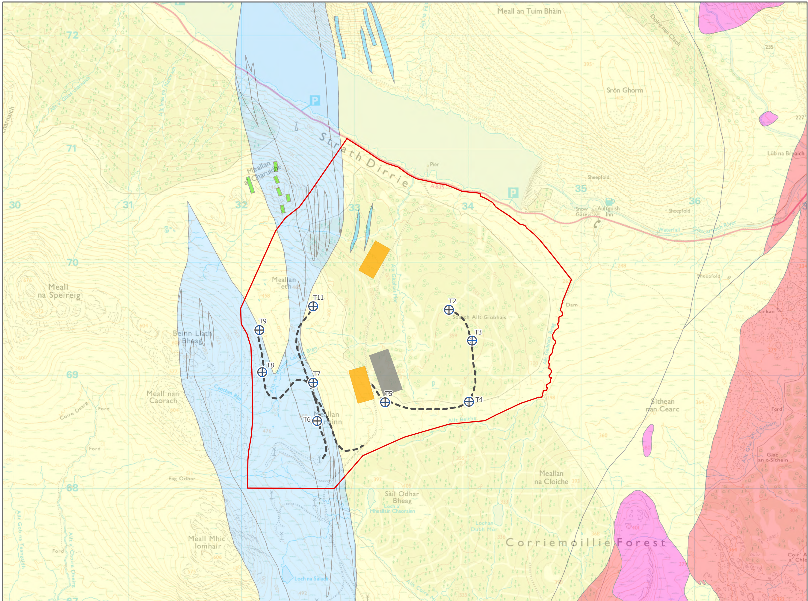
Figure 13.5: Bedrock Geology
